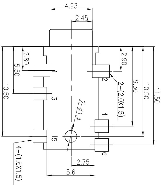
PCB LAYOUT TOP VIEW TOLERANCES:±0.05
